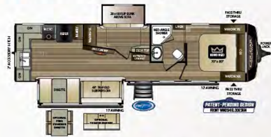
31MBS | Rear kitchen, mid bunkhouse Weight: 7875 LBS. | Length: 35' 3"
