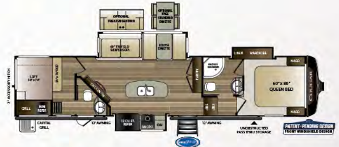
364BHL | 2 bedroom, bath and a half w/ loft Weight: 11225 LBS. | Length: 39' 3"
